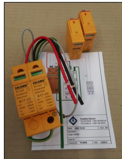
Installed surge arrester in SD75 Cartridge indicator; Green is good, Red is blown
